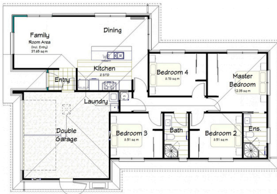
Floor Plan
